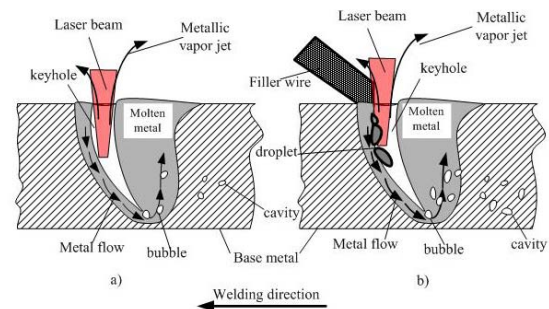
Fig. 4. Cavity formation in laser welding on the board without (a) and with (b) filler wire.
